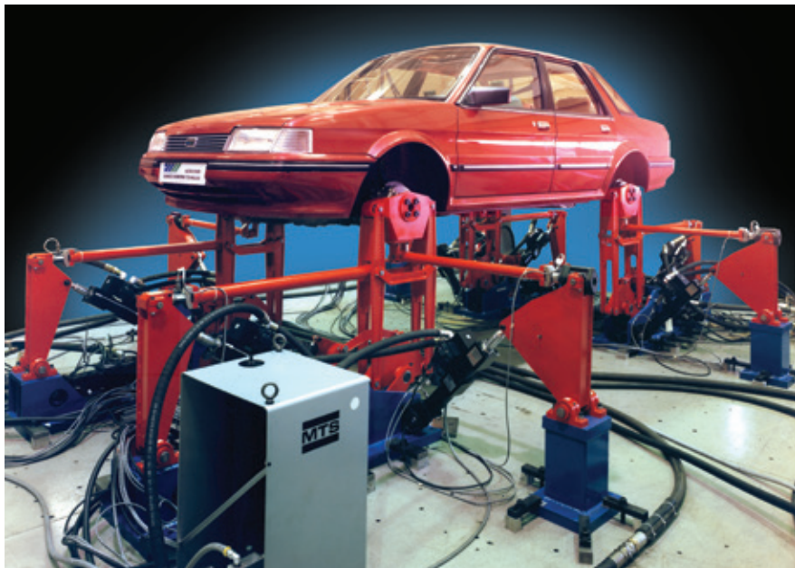
MTS Model 327 4DOF System
