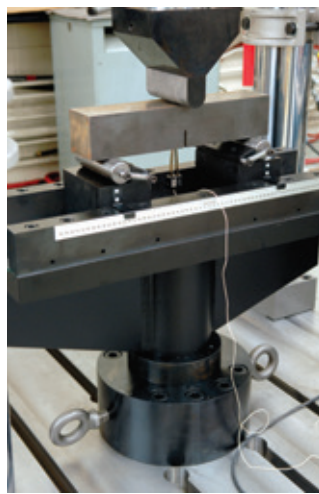
Bend Fixture
