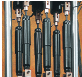
Multi-specimen Fixtures
